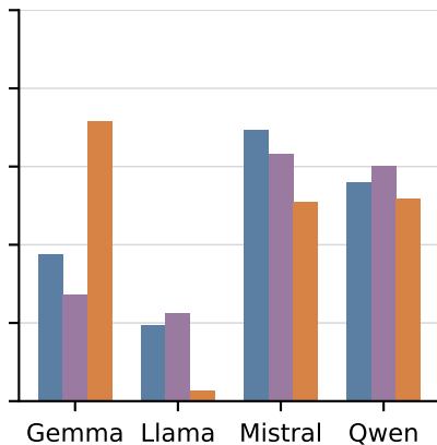
Top-one compliance
