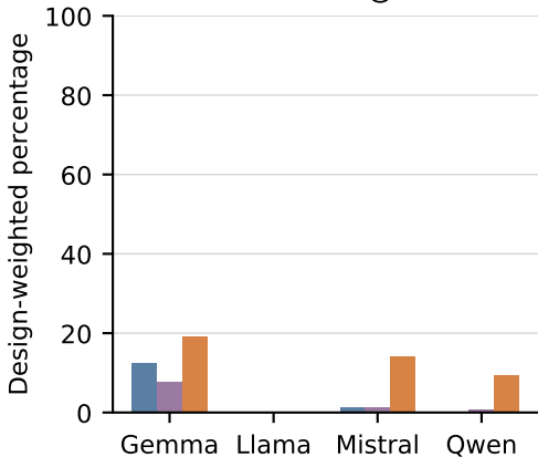
Exact Hit@1
