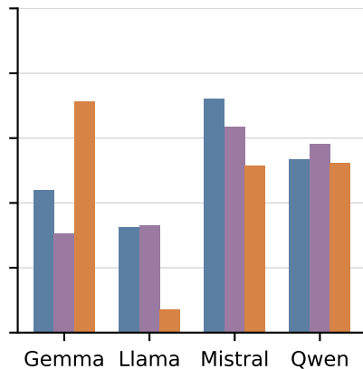
Compliant-list fraction
