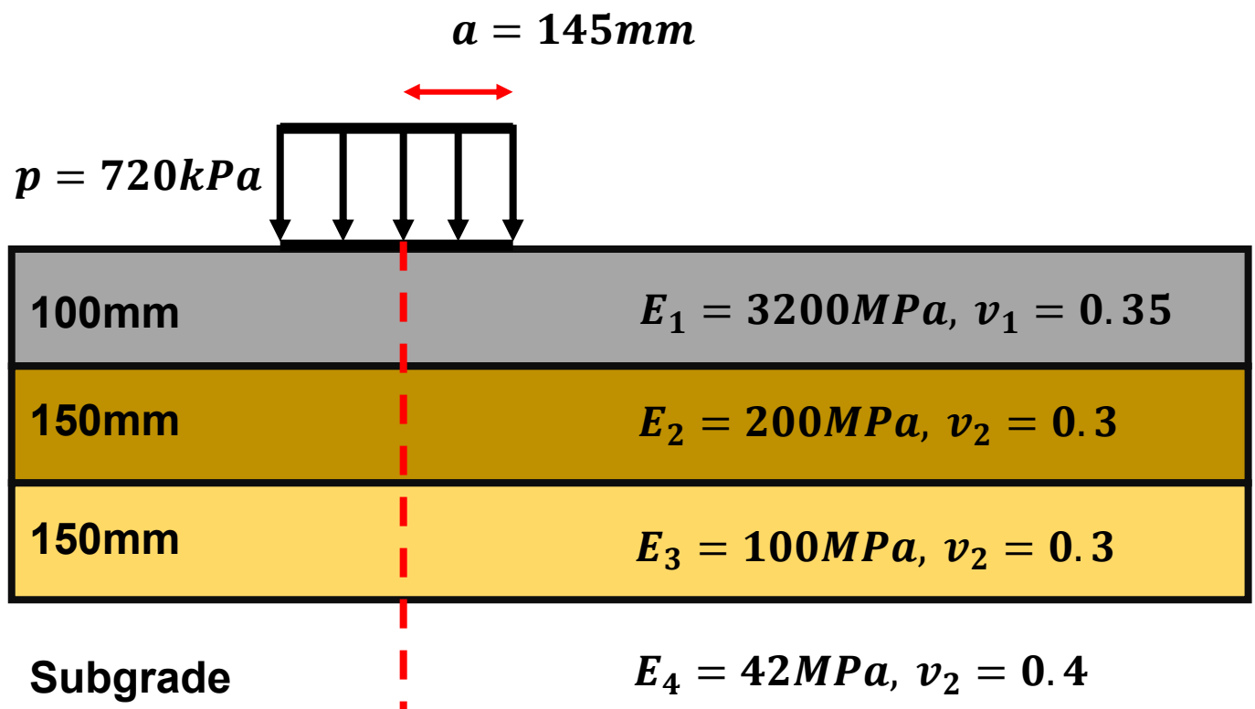
Figure 1. Pavement structure question 3
