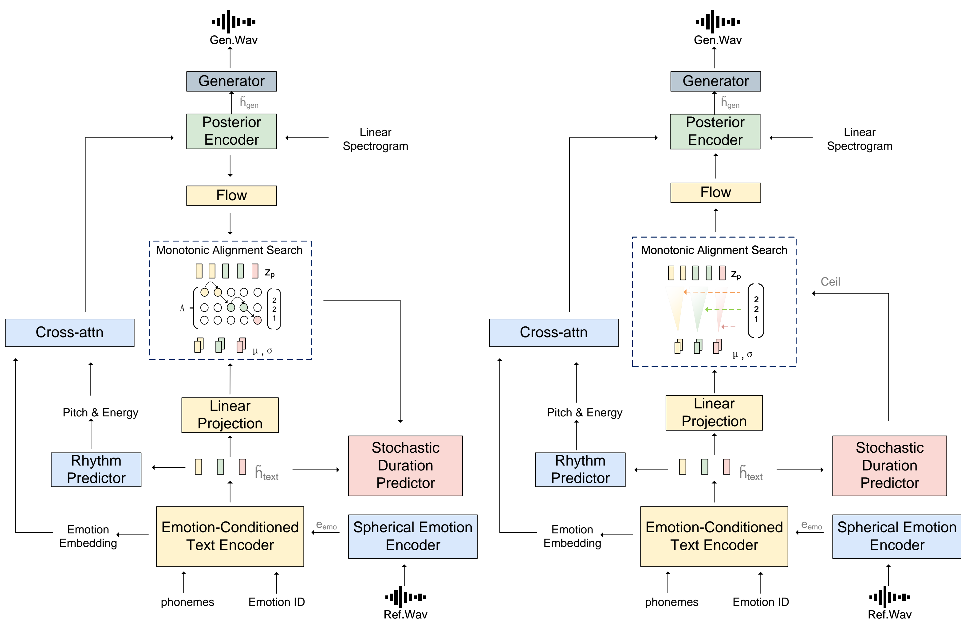
(a) Training procedure
