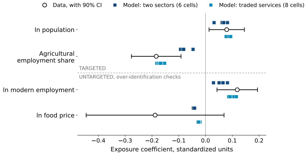
Figure 14: Model fit: targeted and untargeted moments against the data
