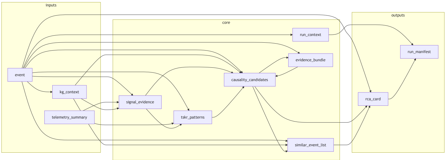
Simplified logical data flow. event is a universal input: its asset_id scopes the KG neighborhood, its timestamp_start/end is the reference interval for all Allen and TSKR scoring, and its event_type and actuation_type are query terms for the similar event search. Optional inputs (SOE, alarms, PM, vendor records, protection logic, etc.) are not shown.
