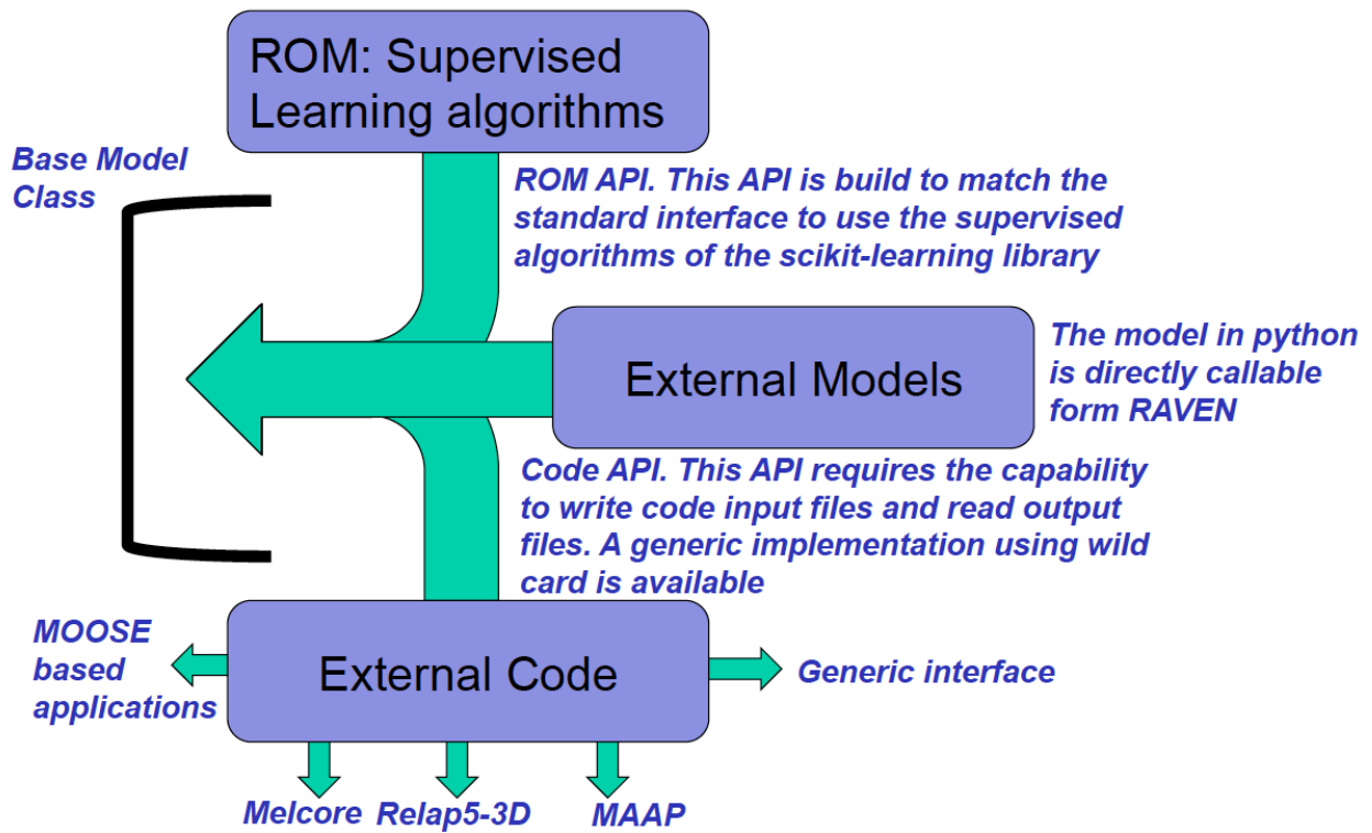
Figure 3. RAVEN Application Programming Interfaces
