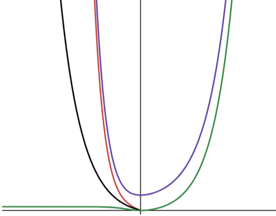
Figure 1: The eigenvalues of the transfer matrix M as a function of J\beta . Since \beta > 0 , the right half of the plane shows the ferromagnetic case while the left half of the plane shows the anti-ferromagnetic for both ferromagnetic ( J = 1 ) and anti-ferromagnetic ( J = -1 ) cases. purple = \lambda_1 , red = \lambda_2 , black = \lambda_3 , green = \lambda_4
