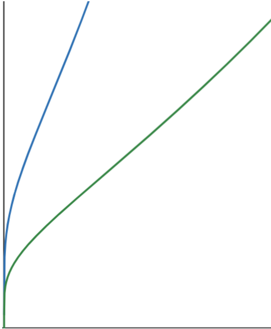
Figure 2: The correlation distance \xi as a function of \beta for both ferromagnetic ( J = 1 ) and anti-ferromagnetic ( J = -1 ) cases. green = ferromagnetic, blue = anti-ferromagnetic
