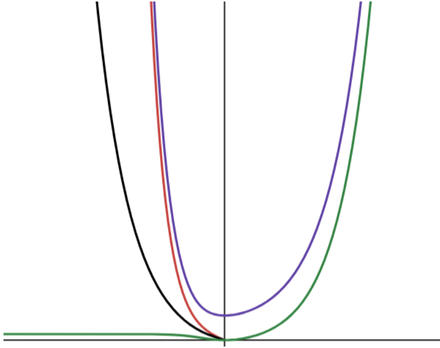
Figure 3: The eigenvalues of the transfer matrix M as a function of J\beta . Since \beta > 0 , the right half of the plane shows the ferromagnetic case while the left half of the plane shows the anti-ferromagnetic for both ferromagnetic ( J = 1 ) and anti-ferromagnetic ( J = -1 ) cases.
