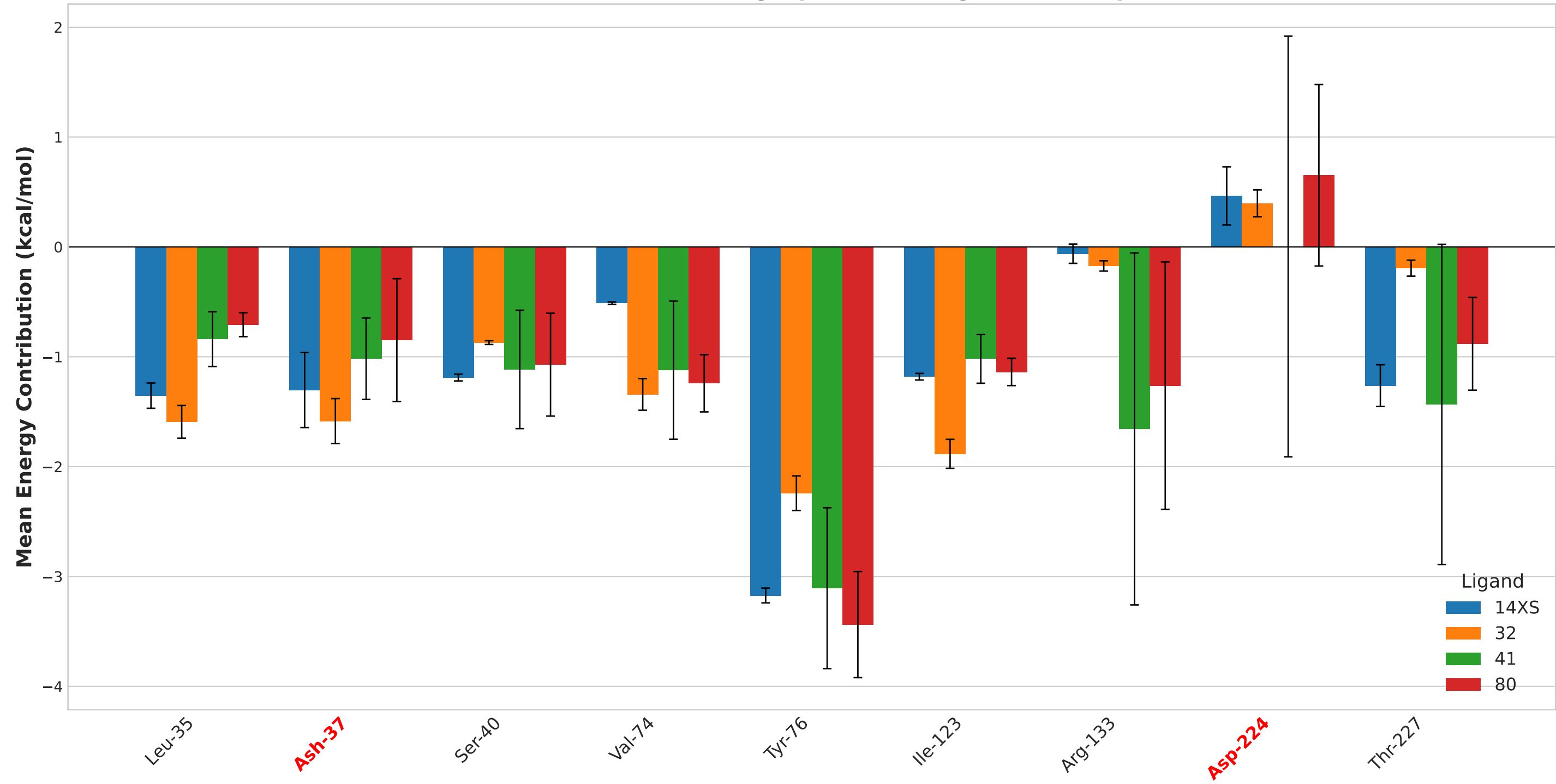
Per-Residue Interaction Fingerprint (Averaged from Triplicates)
