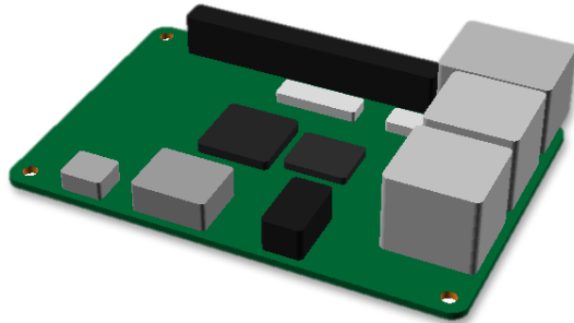
Single-board computer (RPI3-like) - 85.0mm x 56.0mm x 1.4mm PCB with connected components
