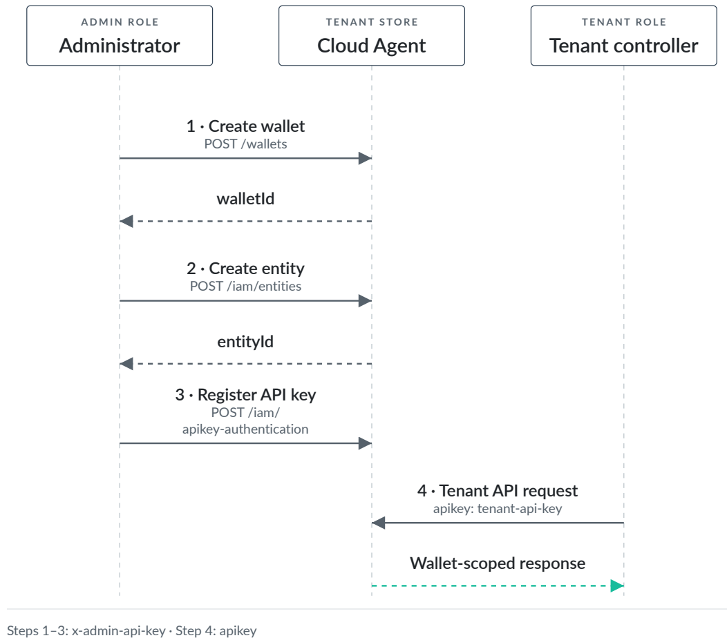
Figure 3: With API_KEY_AUTO_PROVISIONING=false , the administrator creates the wallet, entity, and API key. The tenant API key selects the entity's assigned wallet.
