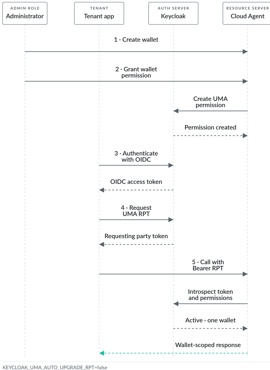
Figure 4: The administrator grants a Keycloak subject access to a Cloud Agent wallet. With automatic RPT upgrade disabled, the tenant controller obtains the RPT. The agent accepts one permitted wallet per tenant request.
