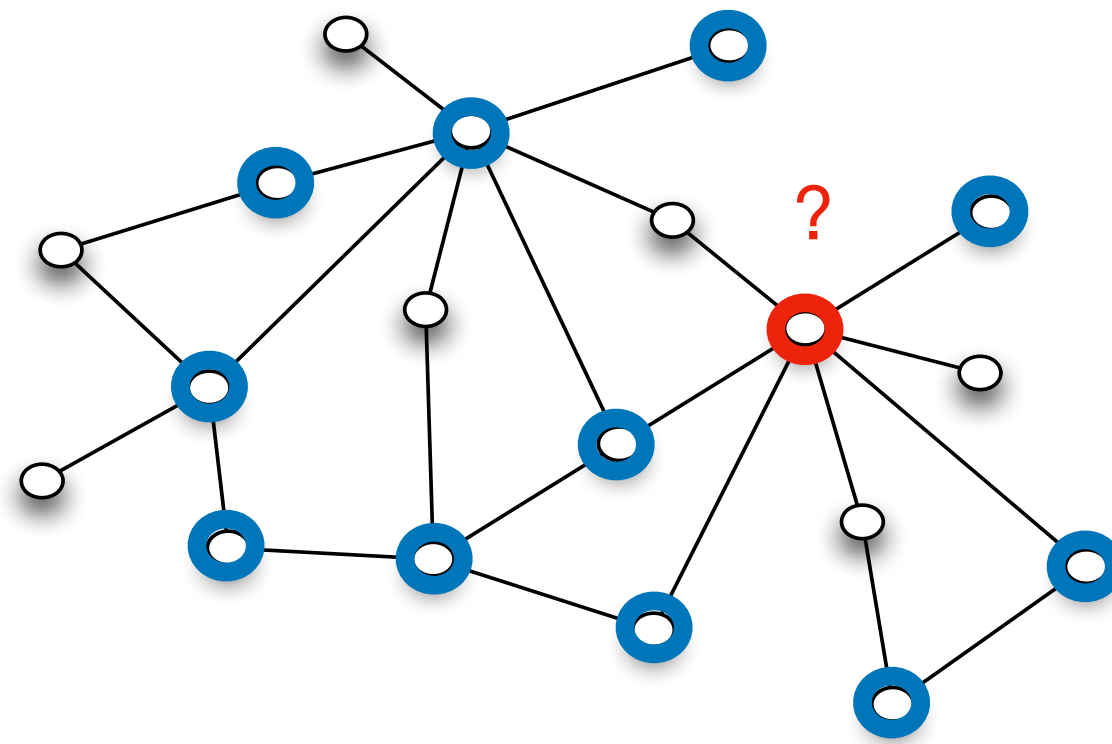
Node classification
