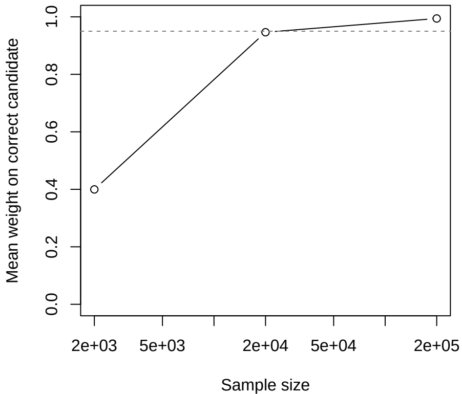
rbf_truth bridge
