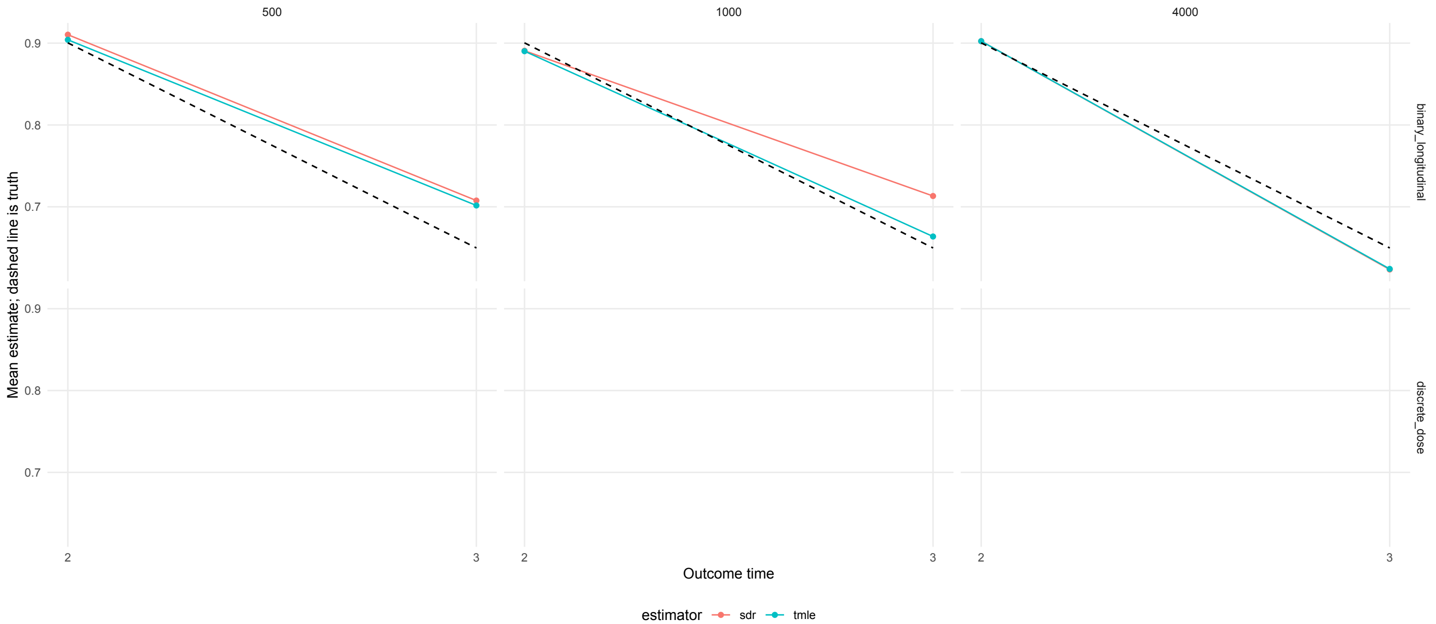
Estimated curves with all four function classes correctly specified
