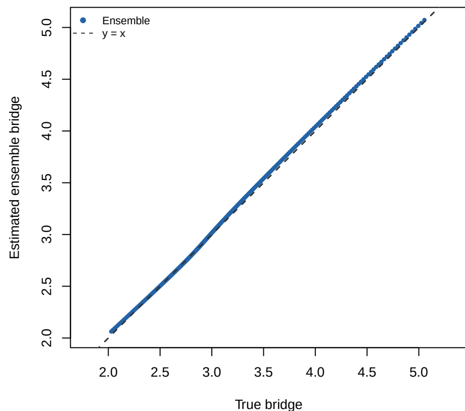
Gaussian kernel truth – bridge
