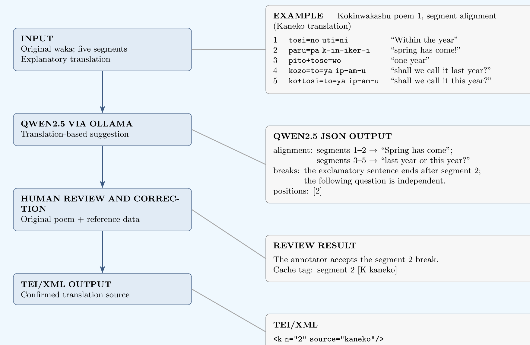
Figure 6: Annotation pipeline from poem and translation, through LLM suggestion and human review, to TEI/XML output.
