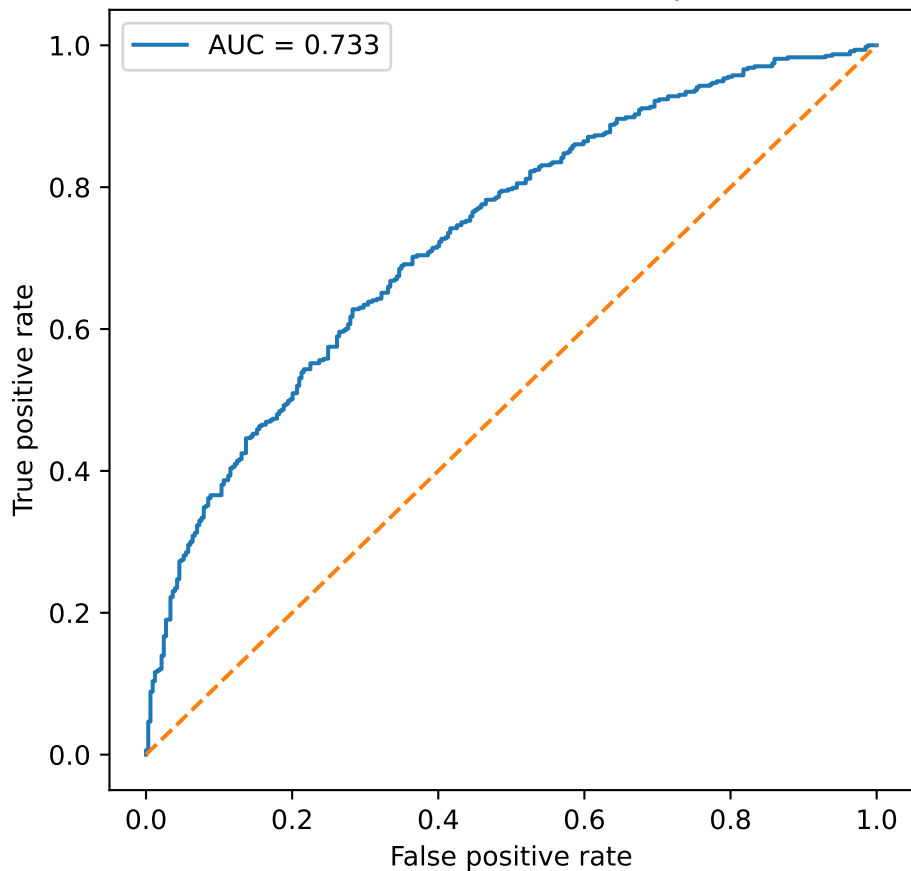
AK4/AK8 candidate BDT pilot
