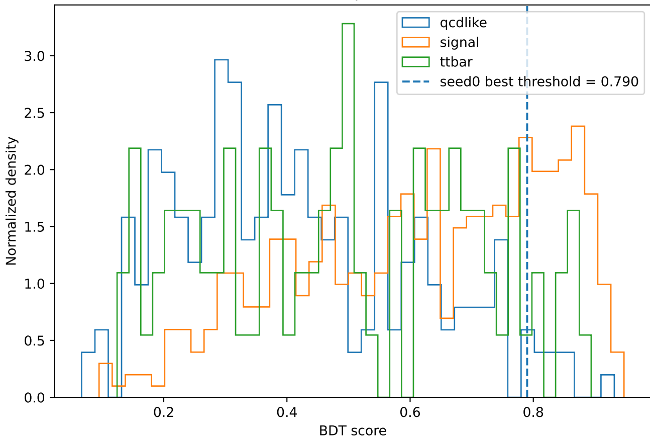
AK4/AK8 candidate BDT pilot: score distributions
