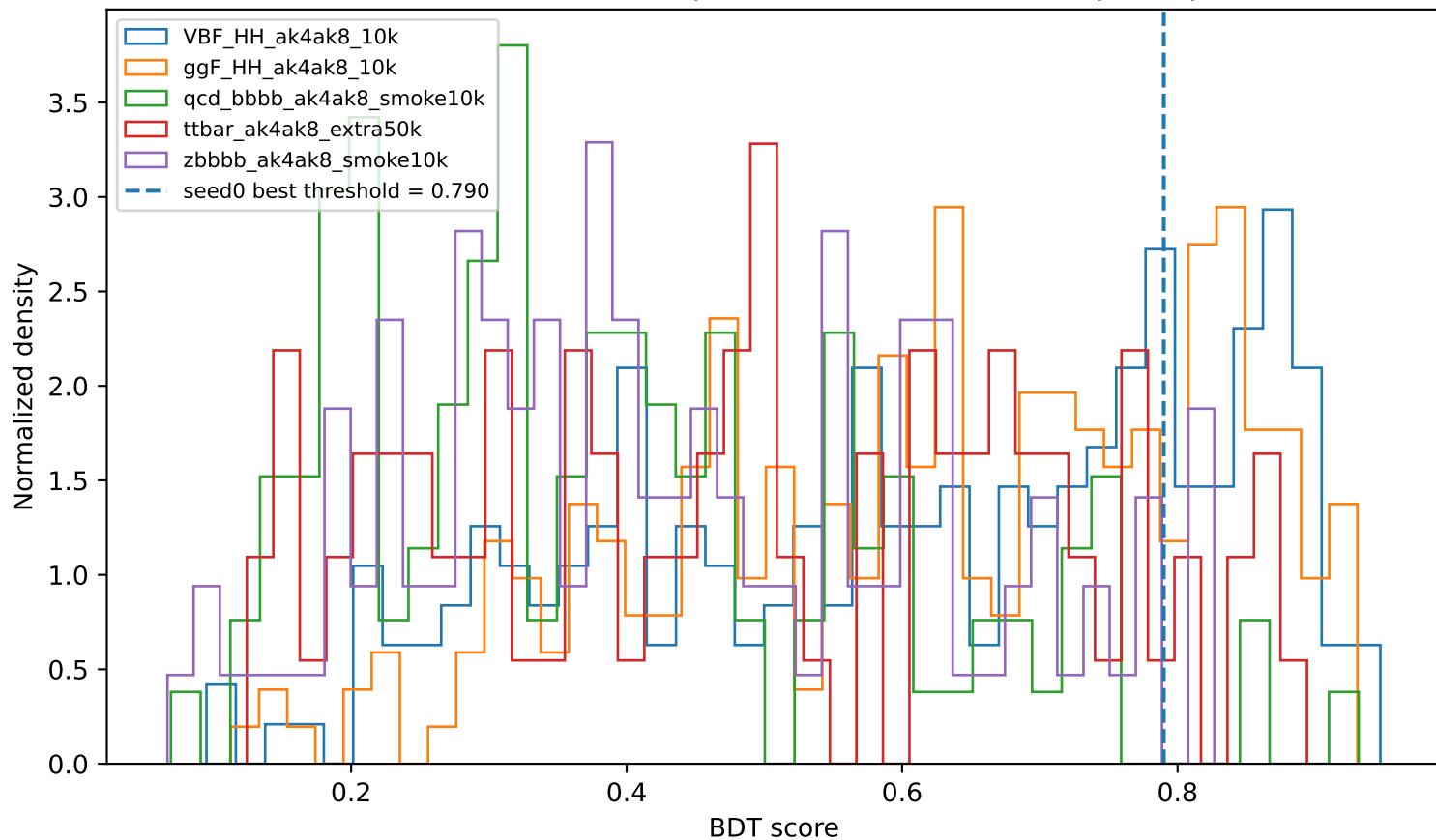
AK4/AK8 candidate BDT pilot: score distributions by sample
