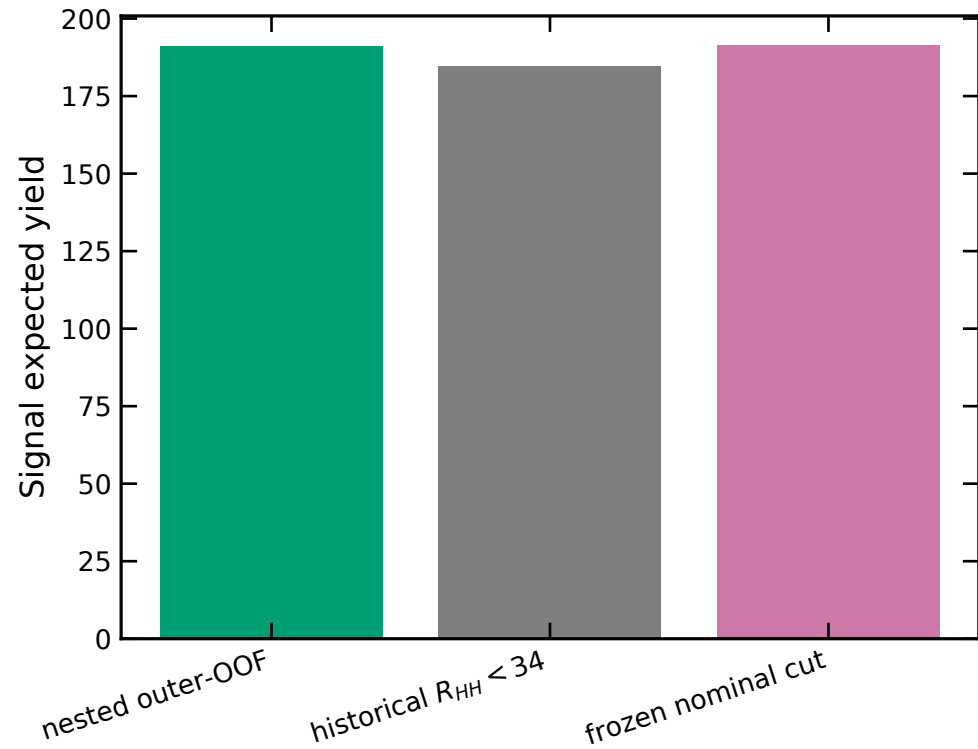
Delphes simulation Run-2 expected-yield projection
