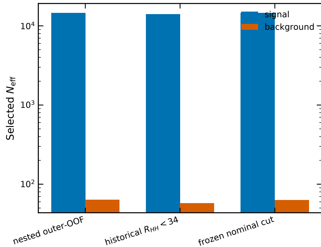
Delphes simulation Pooled category-combined train metrics
