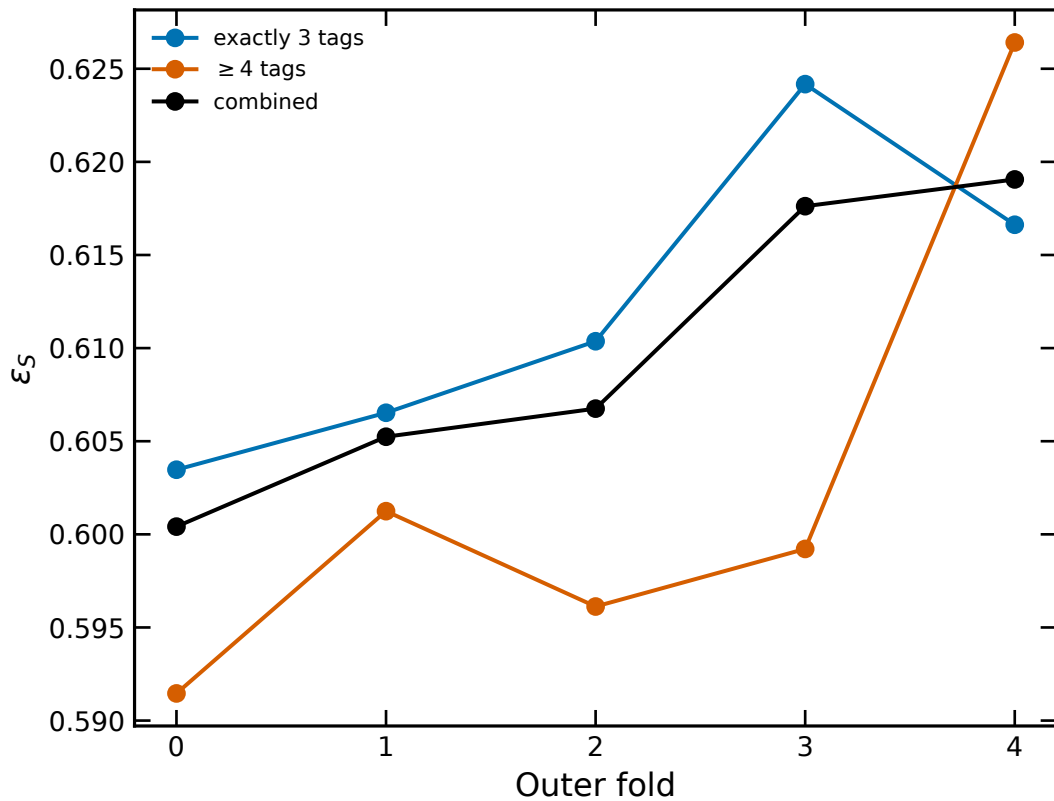
Delphes simulation Primary train-only generalization estimate
