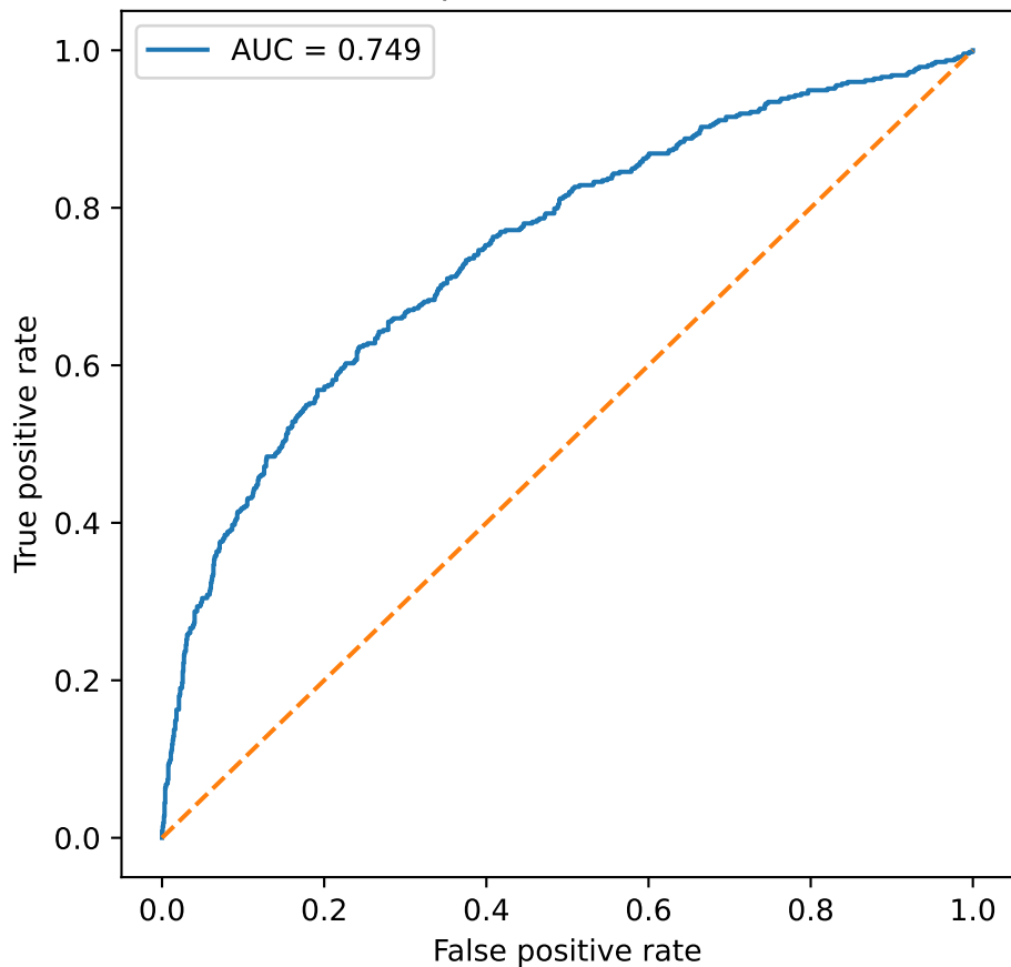
AK4/AK8 expanded candidate BDT v2
