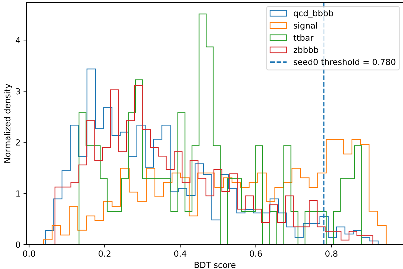
AK4/AK8 expanded candidate BDT v2: score by group
