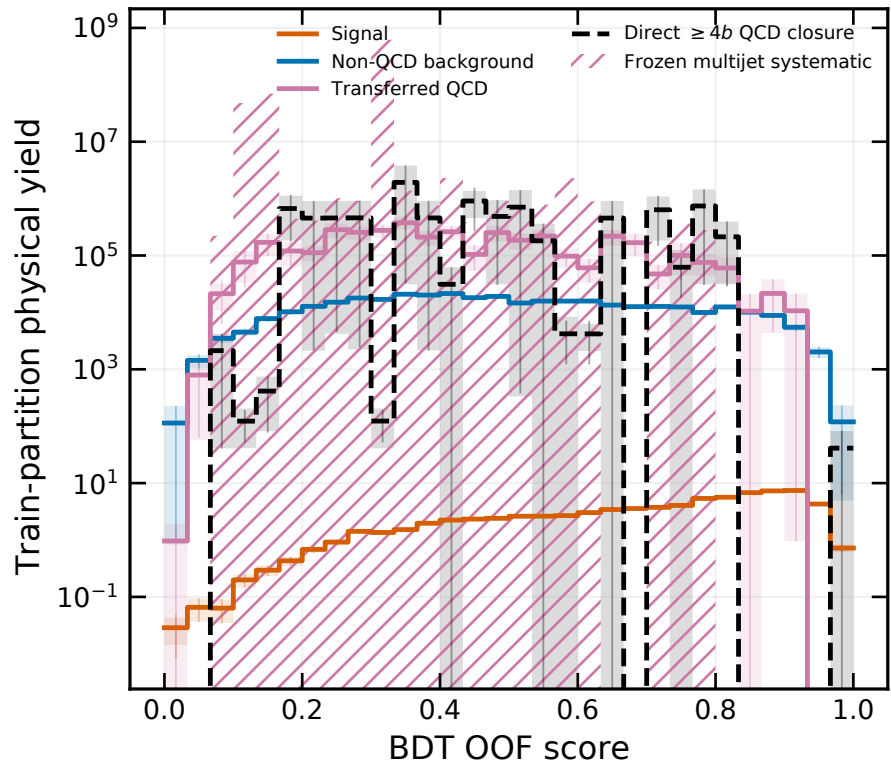
Delphes simulation
