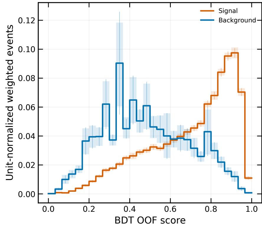
Delphes simulation
