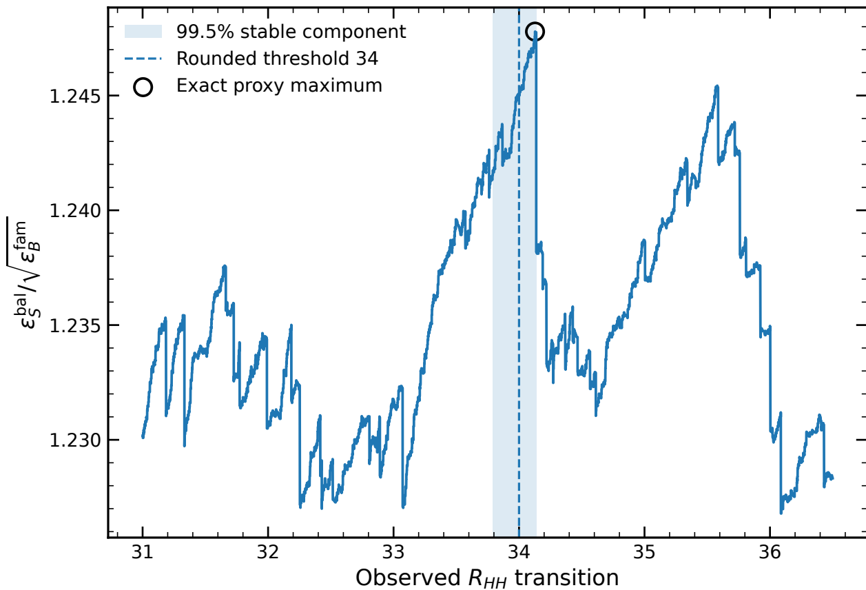
HH \rightarrow b\bar{b}b\bar{b} exact train-only R_{HH} scan
