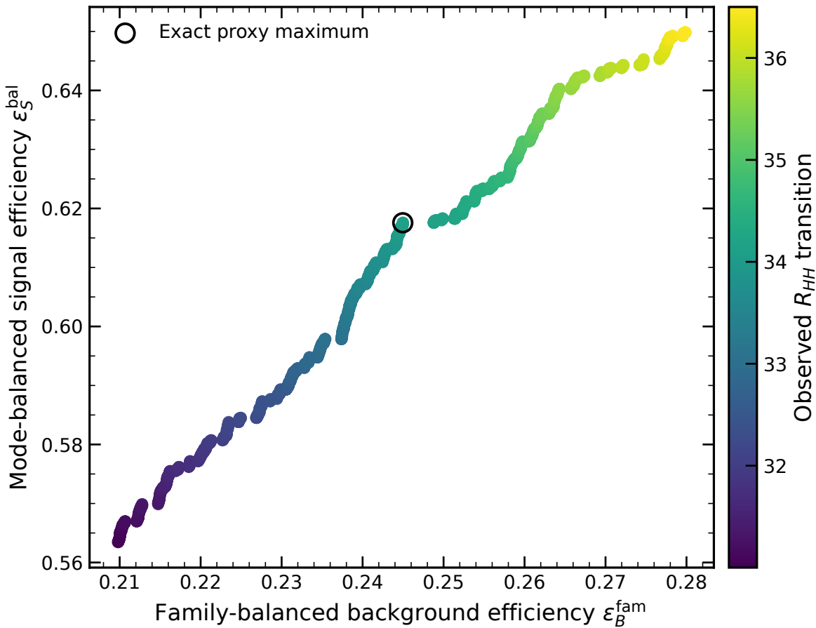
HH \rightarrow b\bar{b}b\bar{b} exact train-only Pareto trajectory
