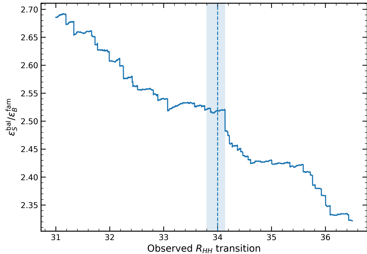
HH \rightarrow b\bar{b}b\bar{b} exact train-only purity proxy
