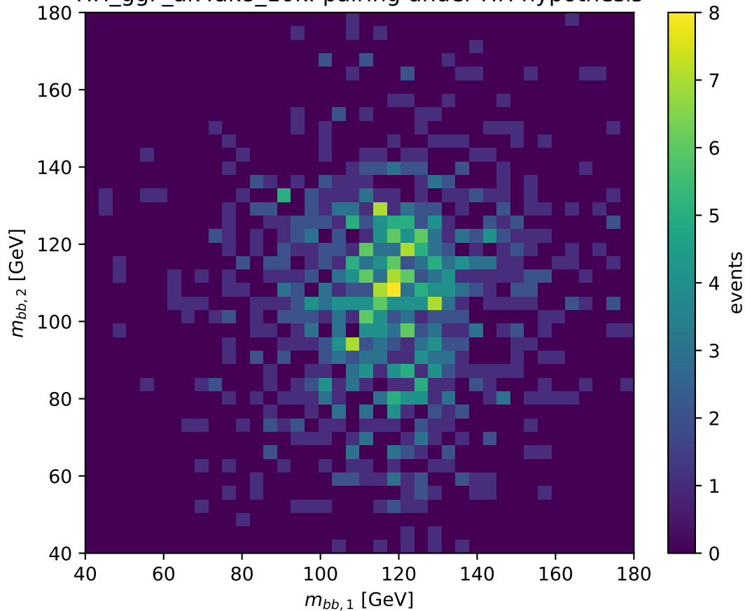
HH_ggF_ak4ak8_10k: pairing under HH hypothesis
