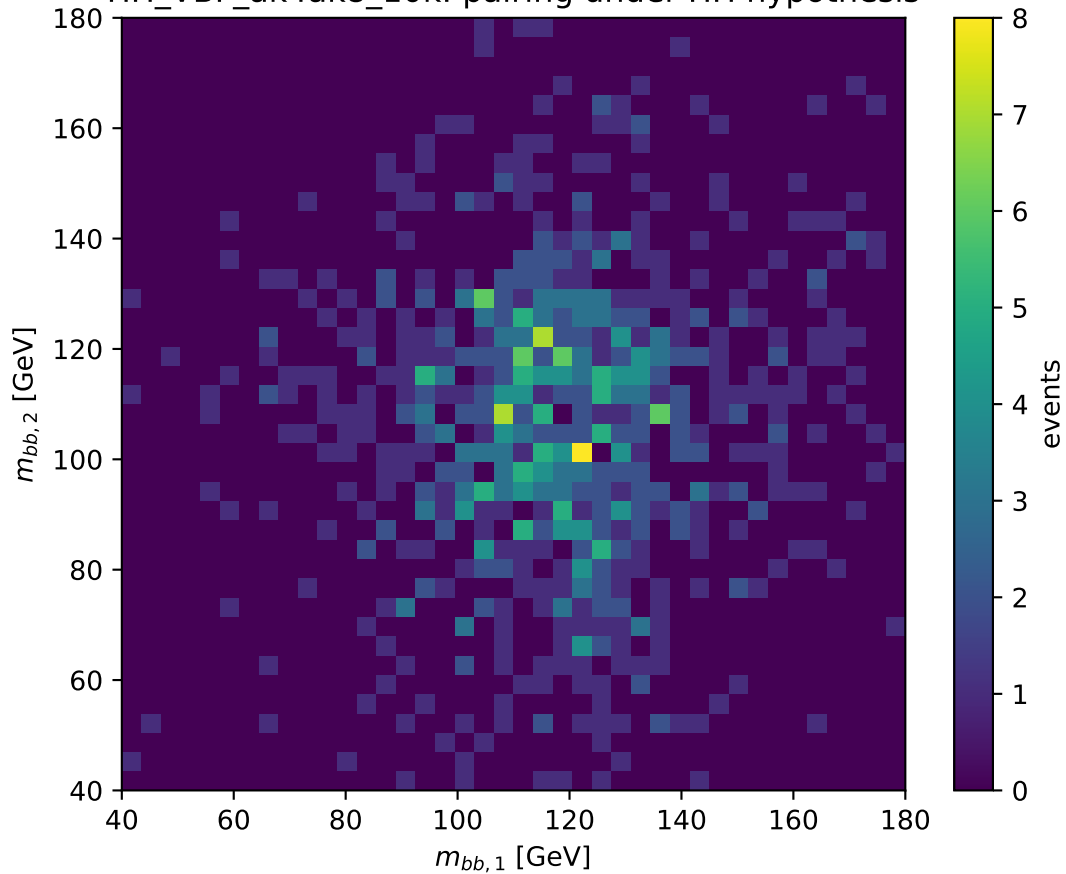
HH_VBF_ak4ak8_10k: pairing under HH hypothesis
