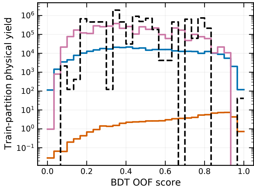
Delphes simulation
