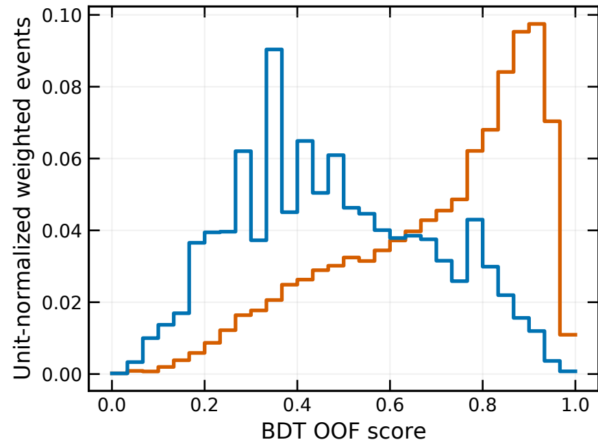
Delphes simulation
