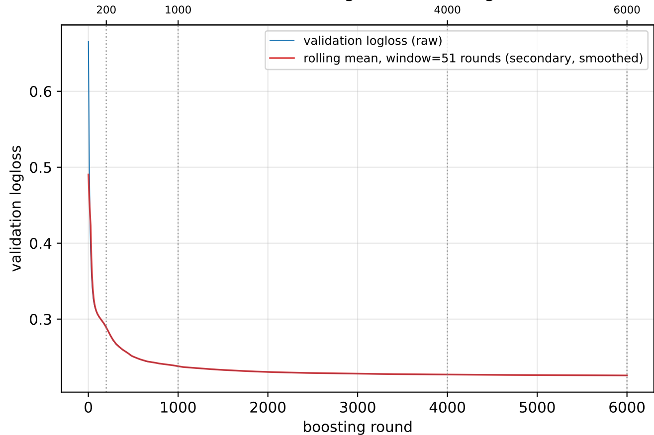
BDT-KF: validation logloss vs boosting round
