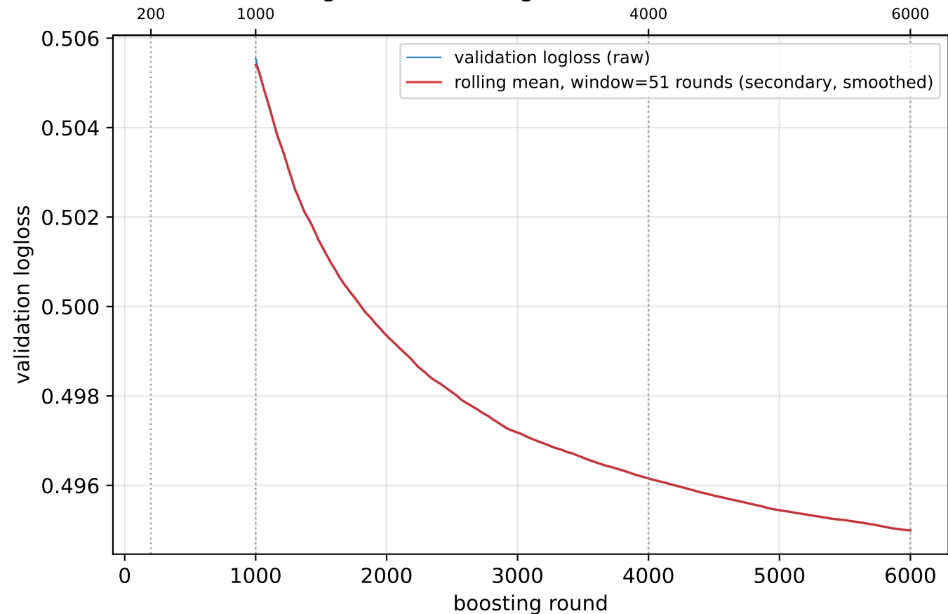
BDT-K: validation logloss vs boosting round (zoomed, rounds 1000-6000)
