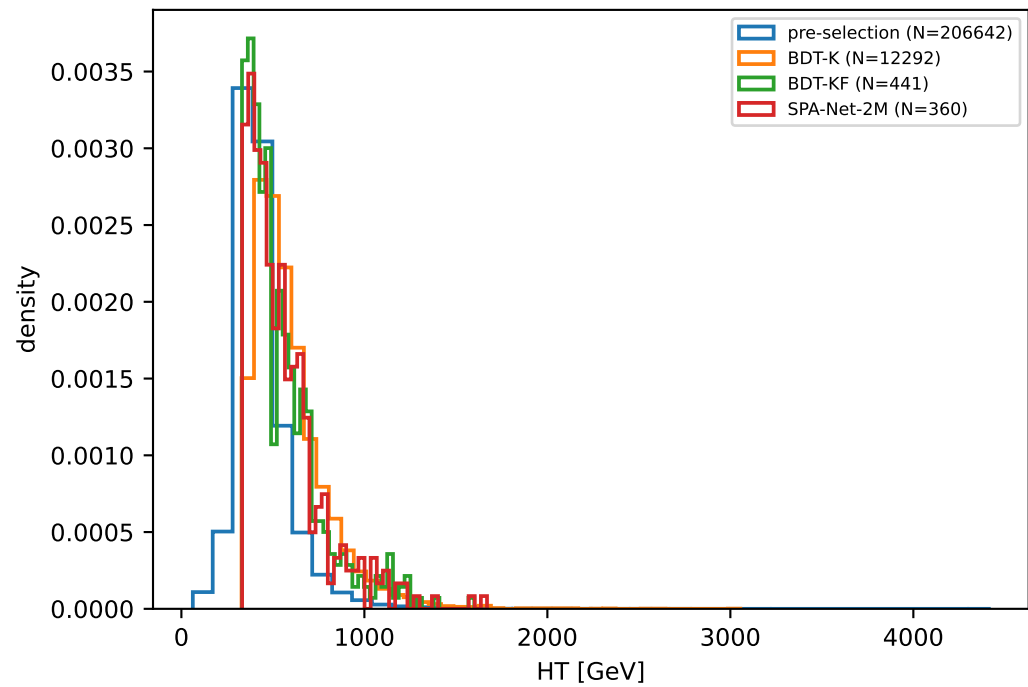
combined_background, \varepsilon_5=0.4 : kinematics & flavor (pre-selection vs K/KF/SPA-2M survivors)
