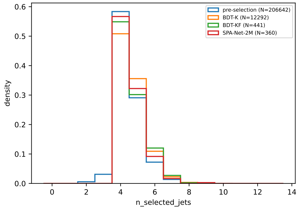
combined_background, \varepsilon_5=0.4 : kinematics & flavor (pre-selection vs K/KF/SPA-2M survivors)
