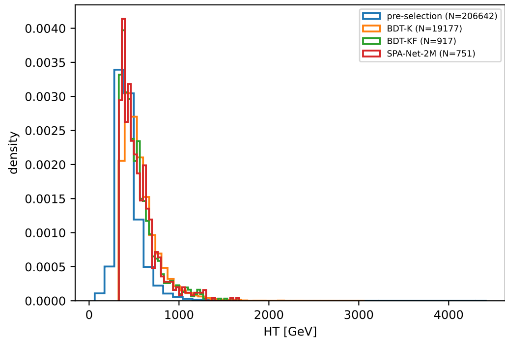
combined_background, \varepsilon_S=0.5 : kinematics & flavor (pre-selection vs K/KF/SPA-2M survivors)
