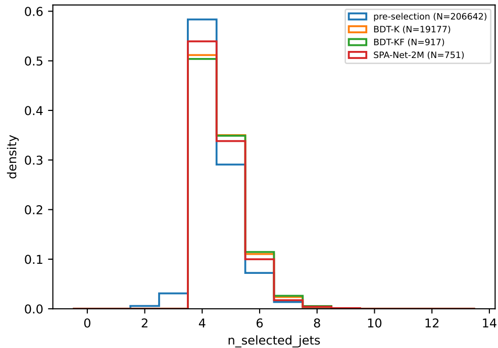
combined_background, \varepsilon_S=0.5 : kinematics & flavor (pre-selection vs K/KF/SPA-2M survivors)
