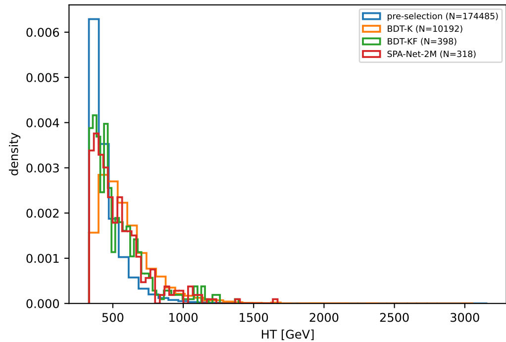
qcd, \varepsilon_S=0.4 : kinematics & flavor (pre-selection vs K/KF/SPA-2M survivors)
