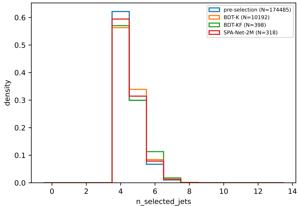
qcd, \varepsilon_S=0.4 : kinematics & flavor (pre-selection vs K/KF/SPA-2M survivors)
