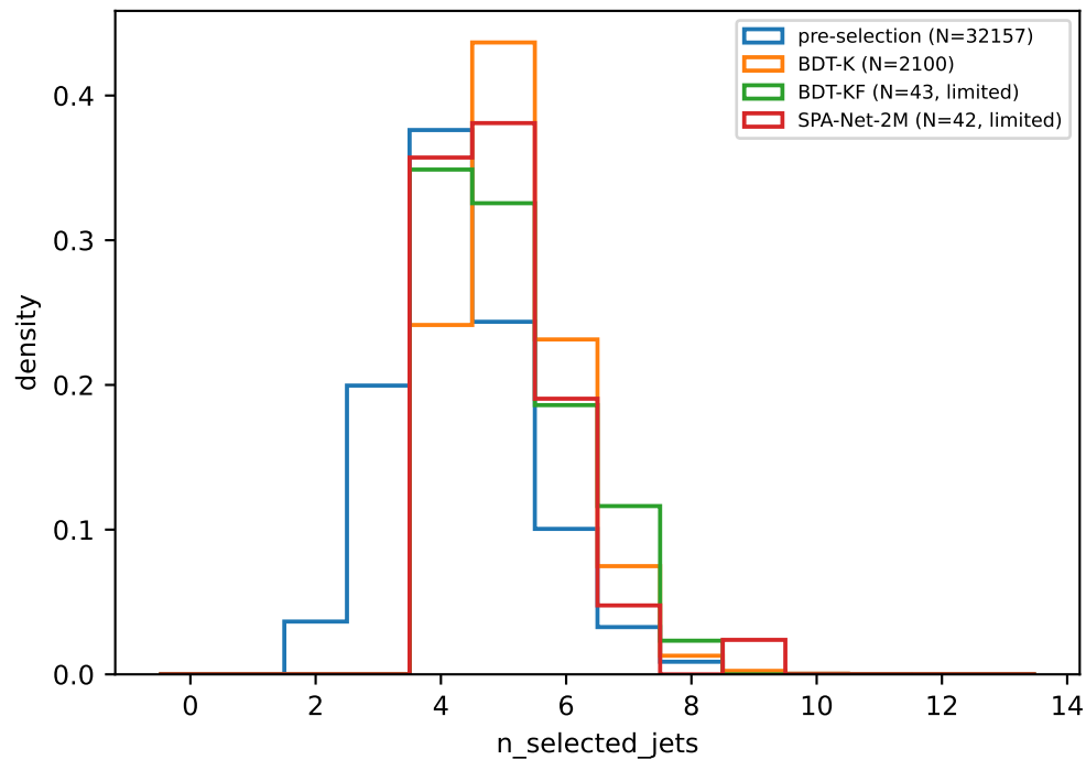
t\bar{t} , \varepsilon_5=0.4 : kinematics & flavor (pre-selection vs K/KF/SPA-2M survivors)
