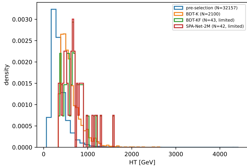
t\bar{t} , \varepsilon_5=0.4 : kinematics & flavor (pre-selection vs K/KF/SPA-2M survivors)
