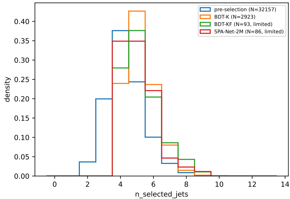
t\bar{t} bar, \varepsilon_5=0.5 : kinematics & flavor (pre-selection vs K/KF/SPA-2M survivors)
