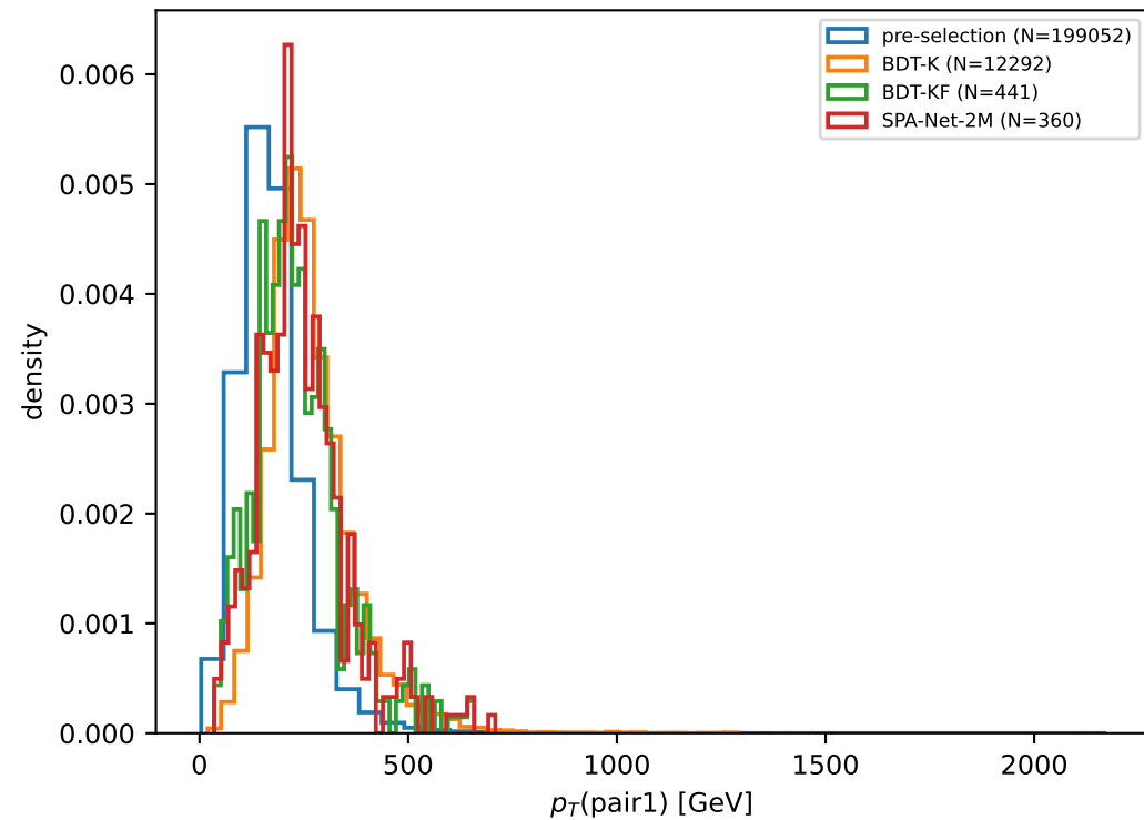
combined_background, \varepsilon_S=0.4 : dijet-pair p_T
