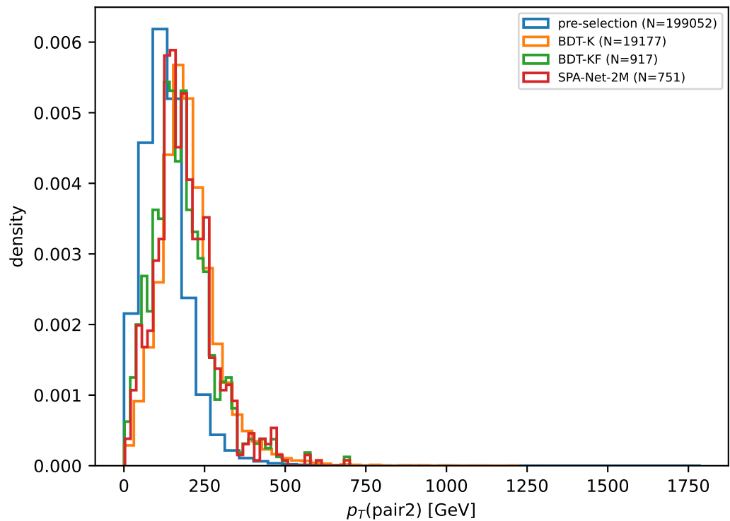
combined_background, \varepsilon_S=0.5 : dijet-pair p_T
