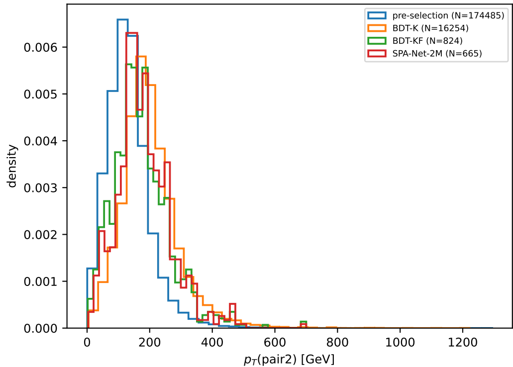
qcd, \varepsilon_S=0.5 : dijet-pair p_T
