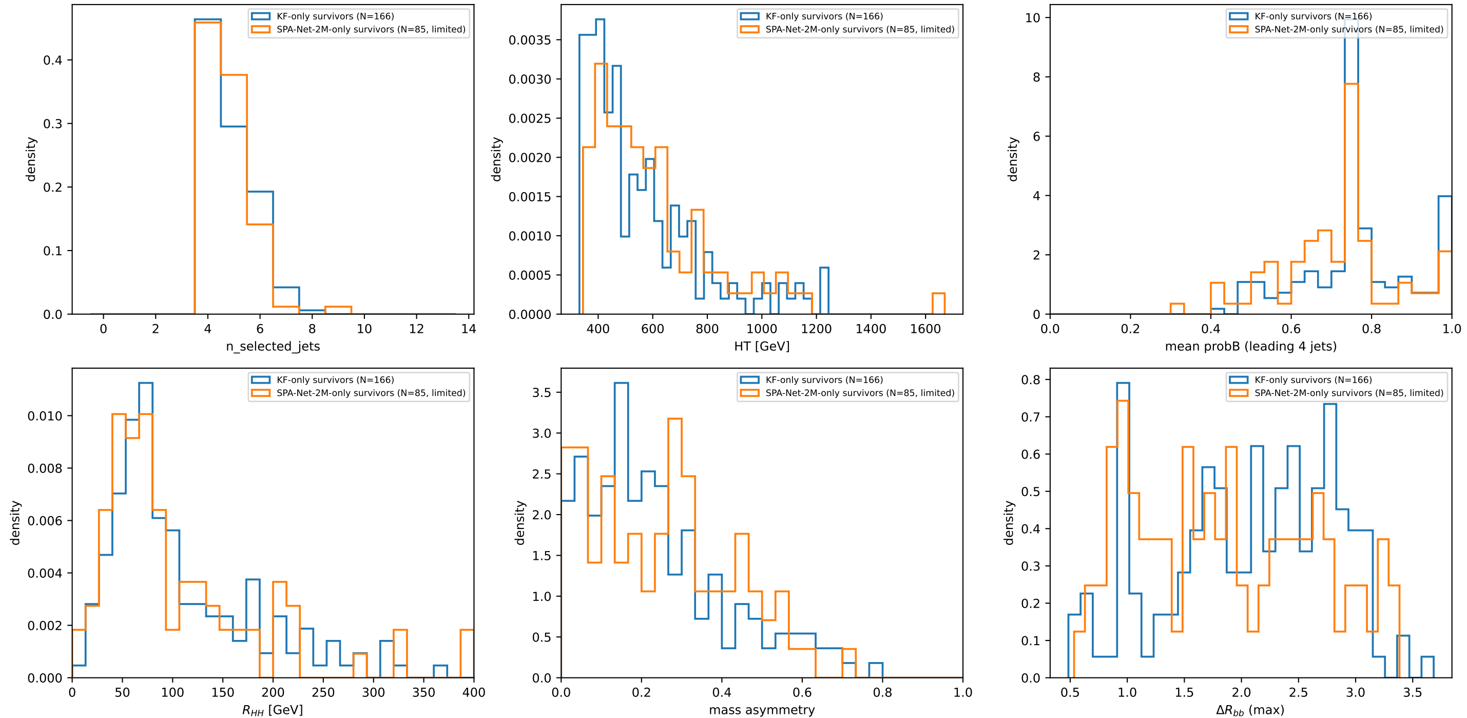
\varepsilon_5=0.4 : KF-only vs SPA-Net-2M-only survivors (combined QCD+ t\bar{t}b\bar{b} background) — observed differences only, no causal claim
