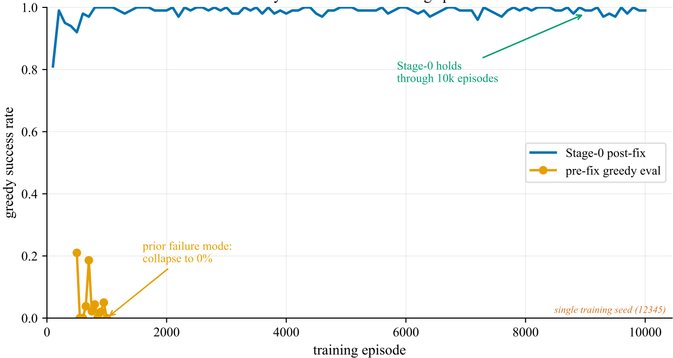
Greedy success rate vs training episode
