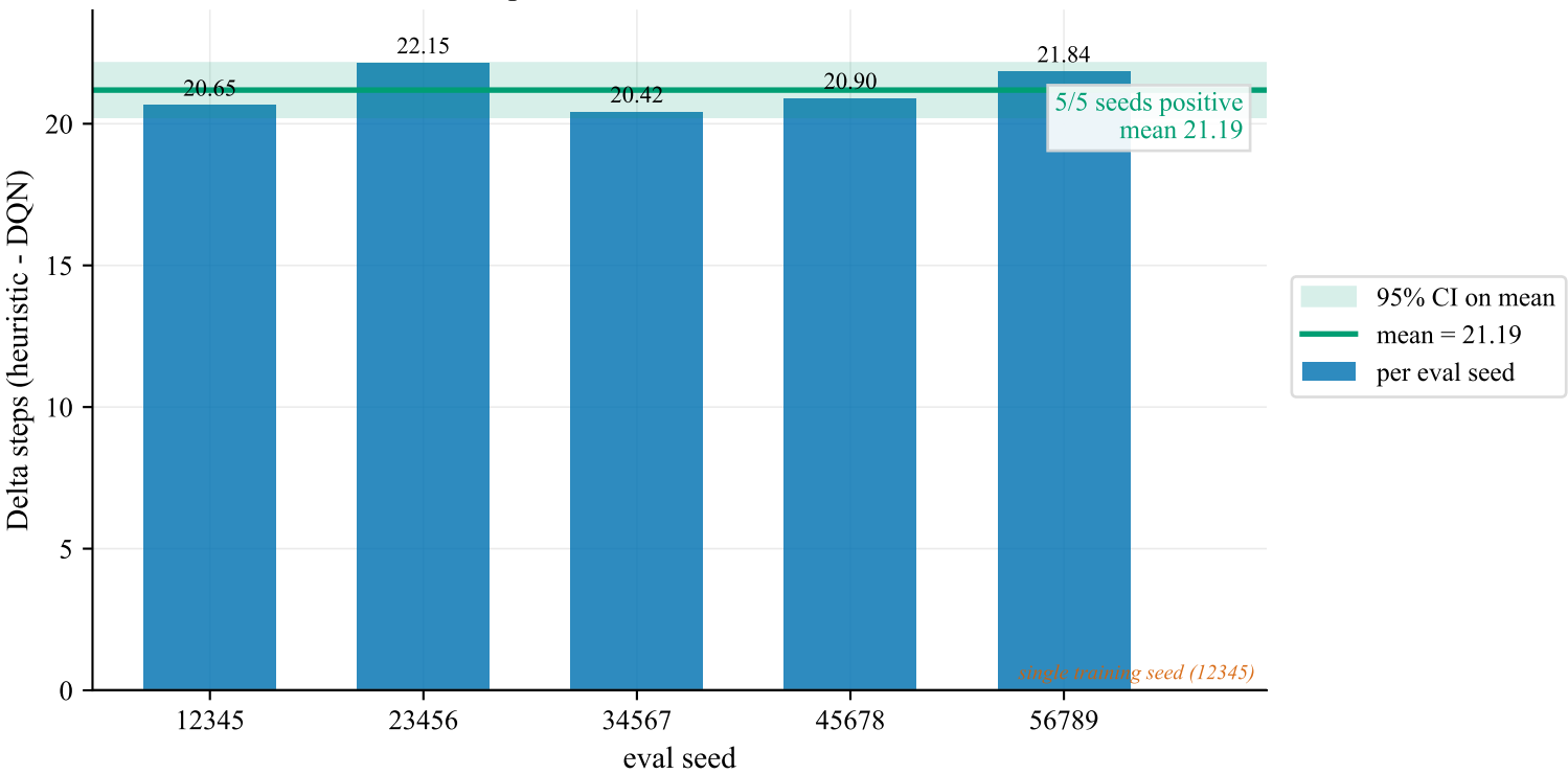
Per-eval-seed paired Delta on shared-solved instances
