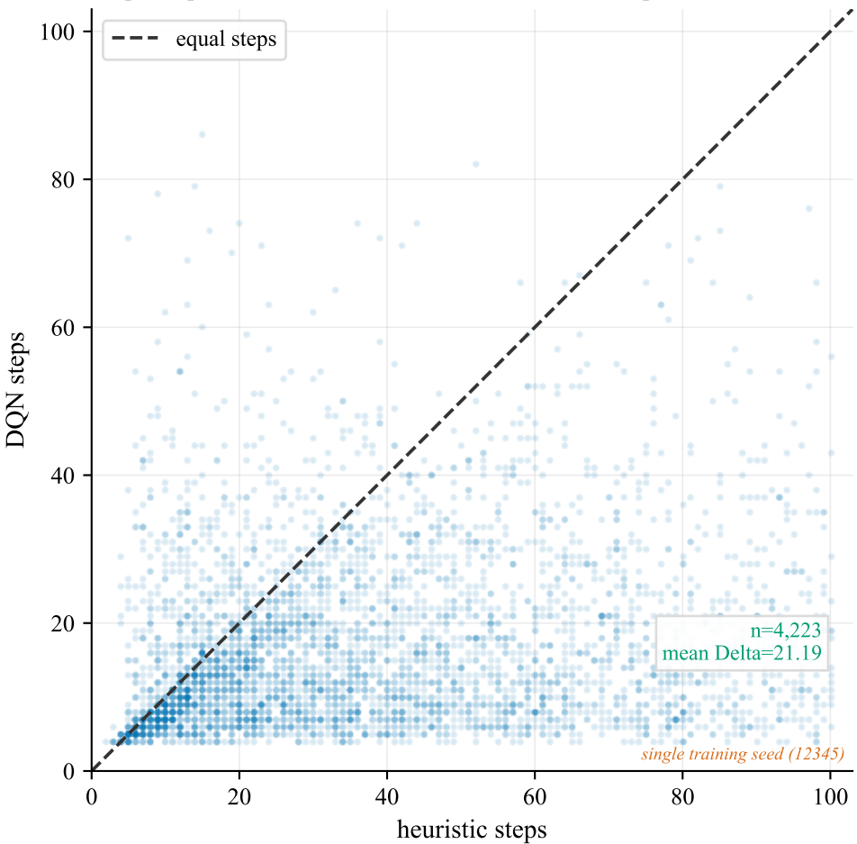
Paired step comparison on shared-solved instances (n=4,223 pooled across 5 eval seeds)
