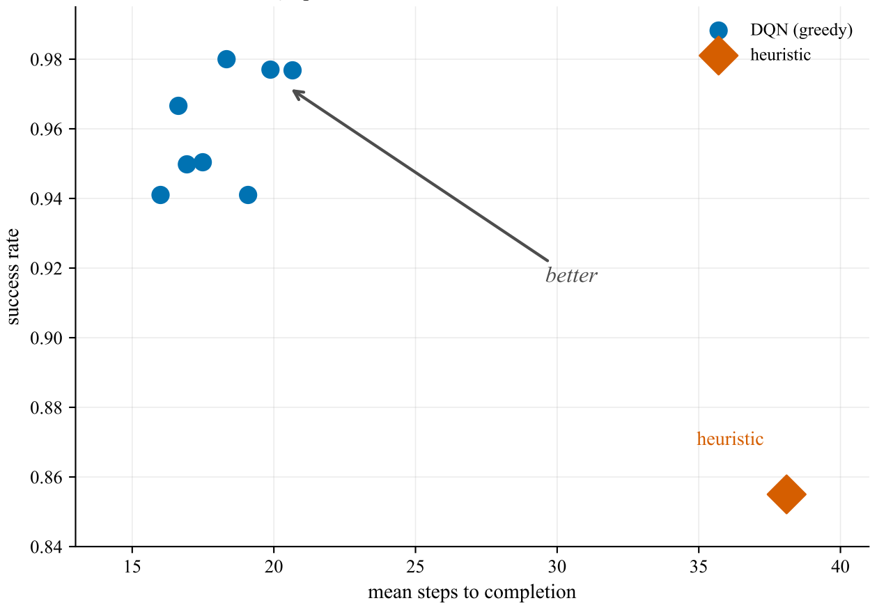
DQN policies dominate the heuristic on both axes
