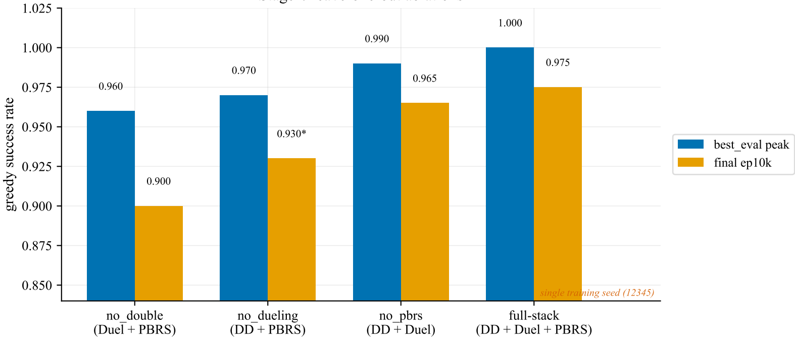
Stage-0 leave-one-out ablations
