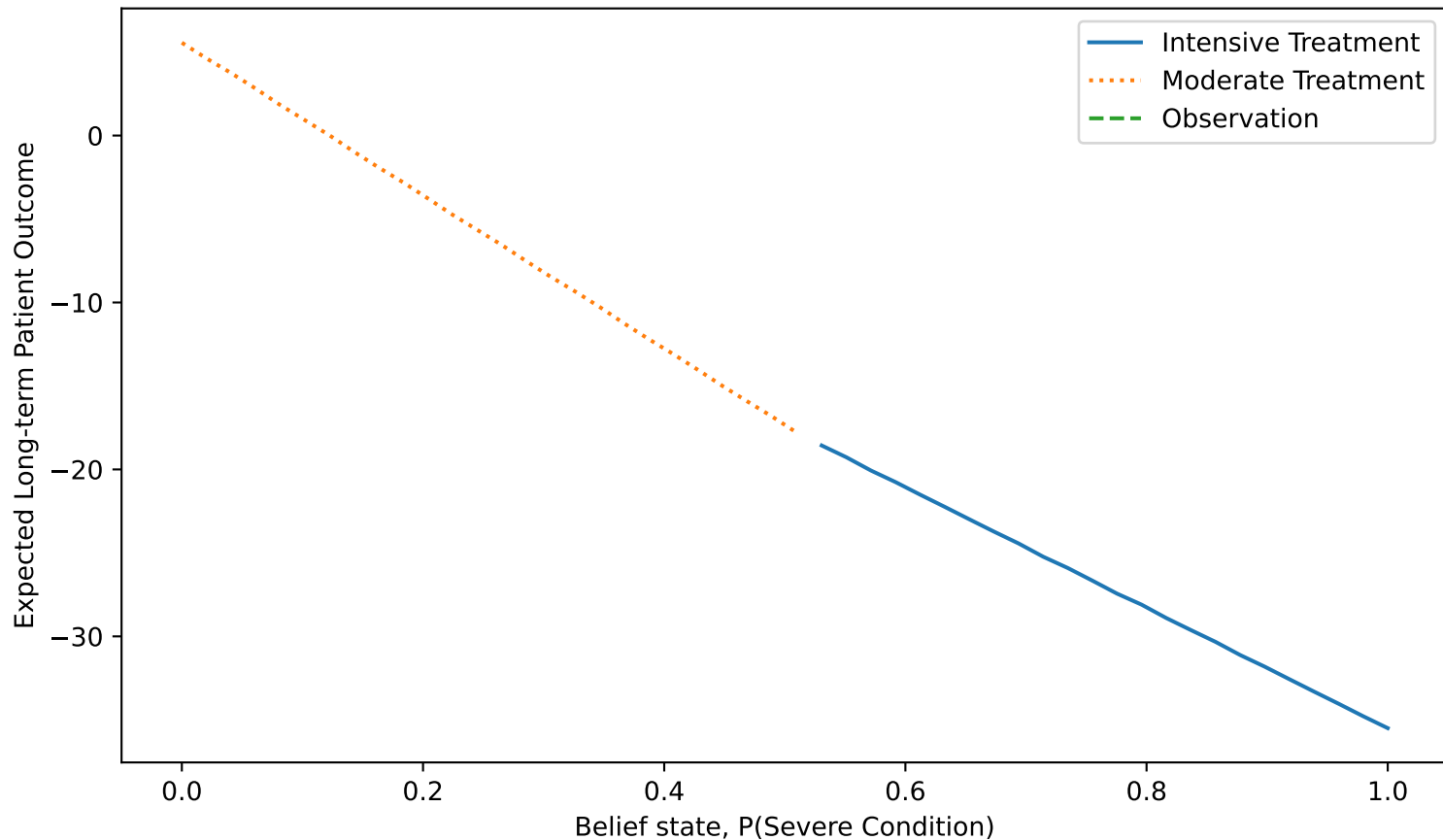
Healthcare Treatment Decision POMDP Solution at Time 1
