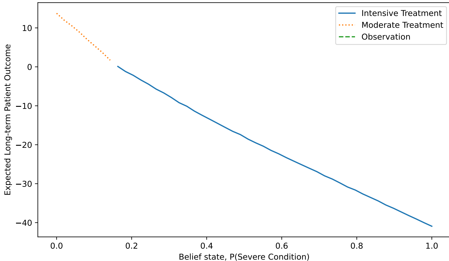
Healthcare Treatment Decision POMDP Solution at Time 10
