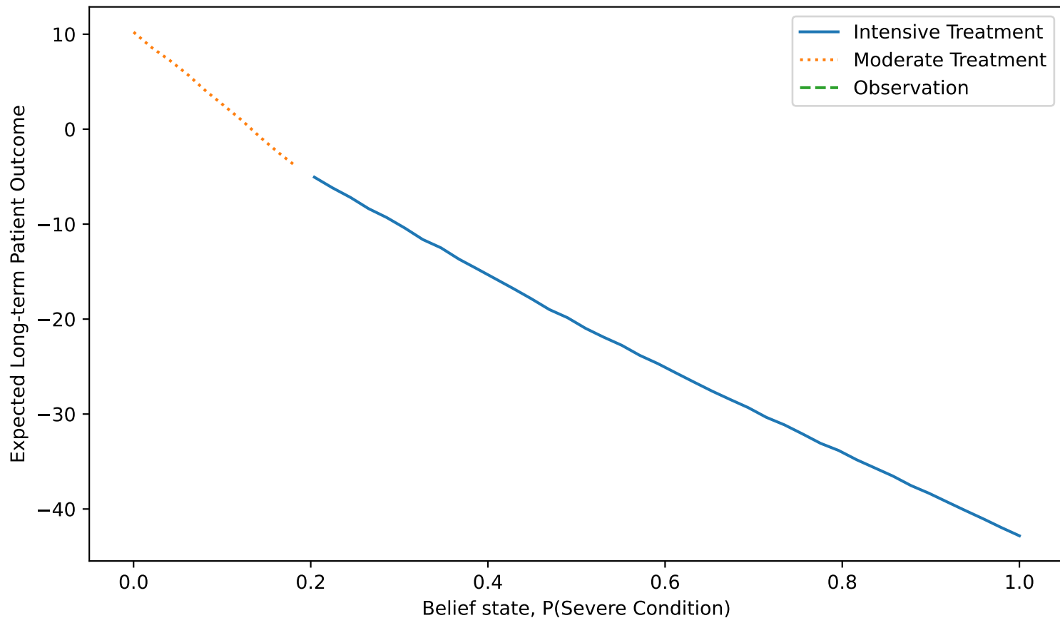
Healthcare Treatment Decision POMDP Solution at Time 5
